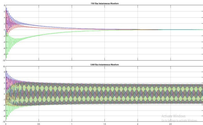
Fig-13: Three phase rotor current and stator current
