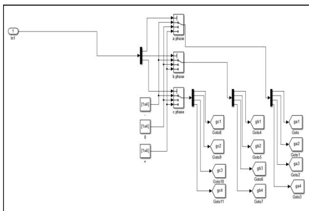
Fig-4: Controller Gate signal generation model in MATLAB Simulink
