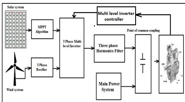
Fig-1: Generalized block diagram of proposed multilevel inverter based solar wind induction motor drive system
