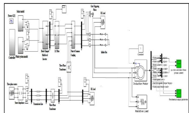
Fig-2: Matlab simulation model of proposed multilevel inverter based induction motor drive
